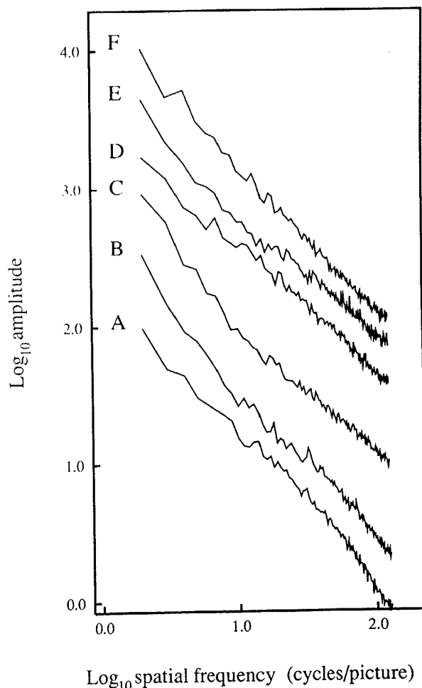
Fig. 8. Amplitude spectra for the six images A-F, averaged across all orientations. The spectra have been shifted up for clarity. On these log-log coordinates the spectra fall off by a factor of roughly 1/f (a slope of -1 ). Therefore the power spectra fall off as 1/f^2 .
