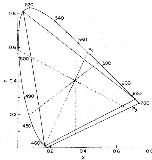
Fig. 1. Chromaticity diagram depicting the eight test directions (shown as dotted lines) and four habituation axes (shown as solid lines) for observer J.K., whose white point is at the intersection of these axes. The provisional cardinal chromatic axes are labeled P_1 (yellowish-bluish) and P_2 (reddish-greenish).
