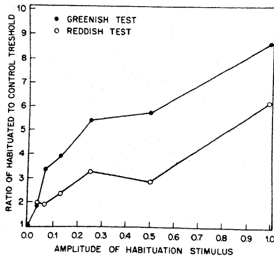
Fig. 4. Effect of amplitude of reddish-greenish sinusoidal habituation on the ratio of the habituated to the control thresholds for detecting reddish (R) and greenish (G) pulses, using the top-up procedure described in the text. Observer: J.K. Mean illuminance: 50 td.
