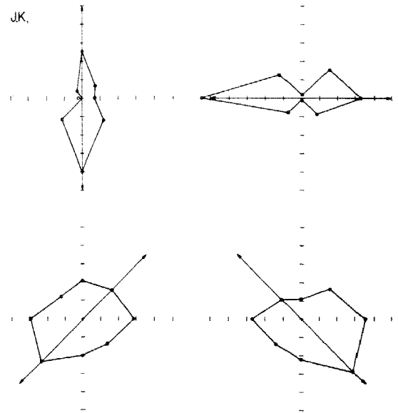
Fig. 5. (Upper) changes in thresholds resulting from viewing fields varying along the provisional cardinal axes. See text for details. Observer: J.K. (Lower) Changes in thresholds resulting from viewing fields varying along directions halfway between the provisional cardinal axes.
