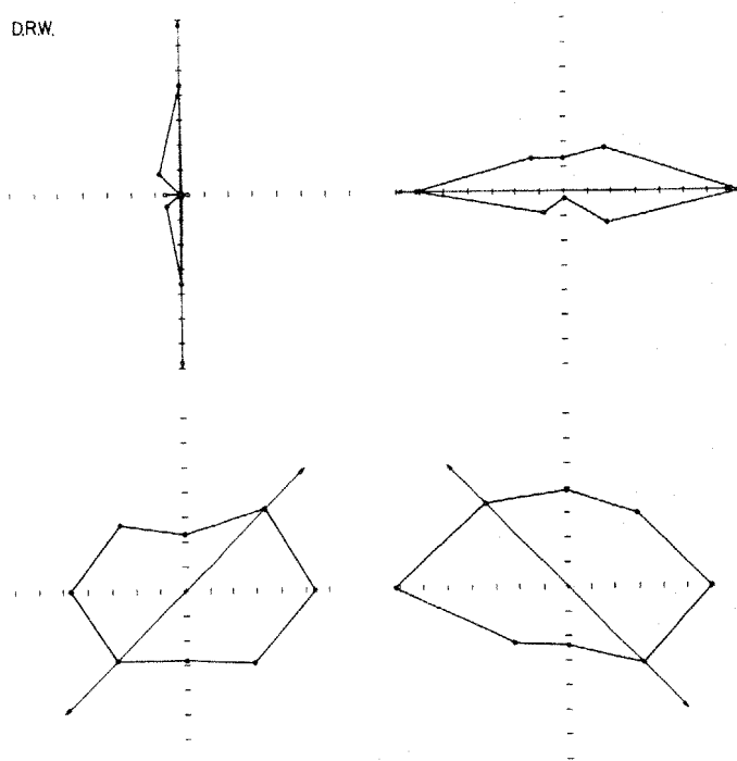
Fig. 7. Effects of purely chromatic (horizontal), purely achromatic (vertical), and mixed habituating stimuli on detectability of test pulses in these same directions for observer D.R.W.
