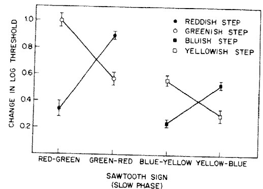
Fig. 8. Changes in thresholds resulting from viewing fields varying in color in a sawtooth fashion as a function of time. Test stimuli step changes in chromaticity. Observer—D.R.W. Mean illuminance = 500 td.
