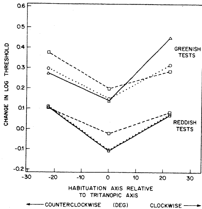
Fig. 10. Effects of three habituation stimuli in the vicinity of tritanopic axis through white on detection of test pulses in the vicinity of the red and green directions. A value of zero on the abscissa corresponds to the tritan line; positive values on the abscissa correspond to clockwise rotation of the adaptation vector in the space defined by our provisional axes. Test stimuli as follows: \square —blueish-red or yellowish-green; \circ —red or green; \triangle —yellowish-red or bluish-green. Results for greenish tests displaced upward by 0.2 log units. Habituation frequency = 1 Hz, gaussian test pulse, standard deviation = 250 msec, total duration = 1500 msec. Mean illuminance = 50 td. Observer—J.K.
