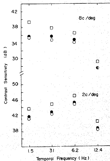
Fig. 2. Contrast sensitivity, defined as the inverse of threshold contrast, for leftward moving \circ , rightward moving \bullet and counterphase gratings \square , as a function of temporal frequency. For counterphase gratings, threshold is expressed in terms of the contrast of either of its moving components. The results of one observer (Peter) at two spatial frequencies are shown.
