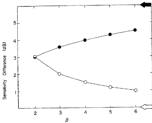
Fig. 1. Values of the decibel difference in sensitivity to moving and counterphase gratings predicted by noisy direction selective mechanisms \circ and noisy non-selective mechanisms \bullet , as a function of the psychometric function slope parameter \beta . Also shown as open and filled arrows are the simple predictions of Levinson and Sekuler.
