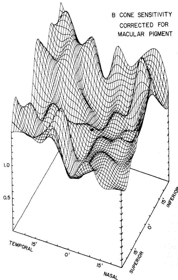
Fig. 7. B cone sensitivity map from Fig. 3 corrected for the absorption of the test flash by macular pigment. Map was obtained by adding macular pigment density shown in Fig. 6 to B cone sensitivity map of Fig. 3.
