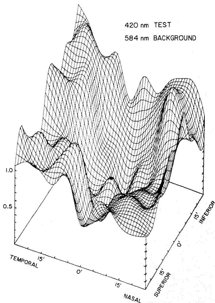
Fig. 3. Sensitivity map for D.R.W. using a 1.1' , 420 nm, 50 msec test flash in locations spaced 5' of arc apart presented against a 2.8 log td 584 nm background. For this and other figures like it for D.R.W., the left corner of the plot represents the superior temporal fovea; the far corner represents the inferior temporal fovea; center of fixation is represented by black dot. Hatchmarks along base of plot indicate divisions of 5' of arc. Hatchmarks along sides of plot indicate 0.1 log units in sensitivity. A value of 0.0 corresponds to 6.4 log quanta/flash.
