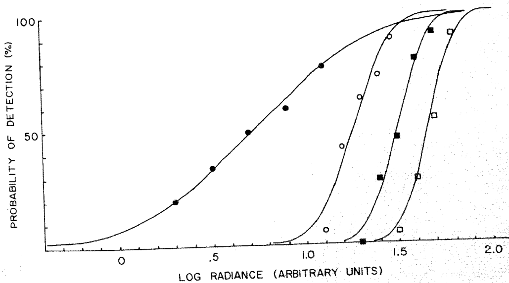
Fig. 11. Frequency of seeing curves for A.L.N. obtained with a 1.1' test flash seen by B cones (solid circles), a 1.1' test flash seen by G cones (open circles), and 15' flash seen by B cones (solid squares), and a 15' flash seen by G cones (open squares).
