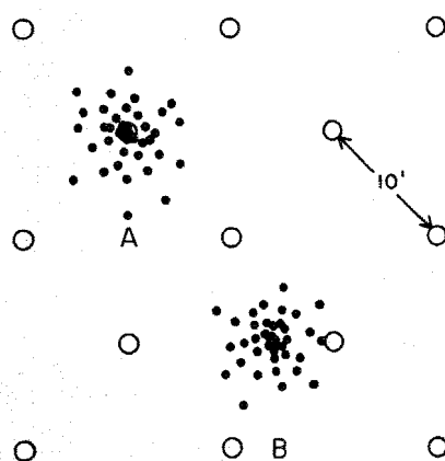
Fig. 12. Array of B cones in the punctate sensitivity model. B cones, shown as open circles, are spaced 10' of arc apart in a rectangular array. In (A), the mean location from flash to flash of the center of the light distribution lies on a cone, whereas in (B) the mean location lies 4' from the nearest cone. Dots represent the locations of individual test flashes which vary in accordance with the distribution of eye positions.
