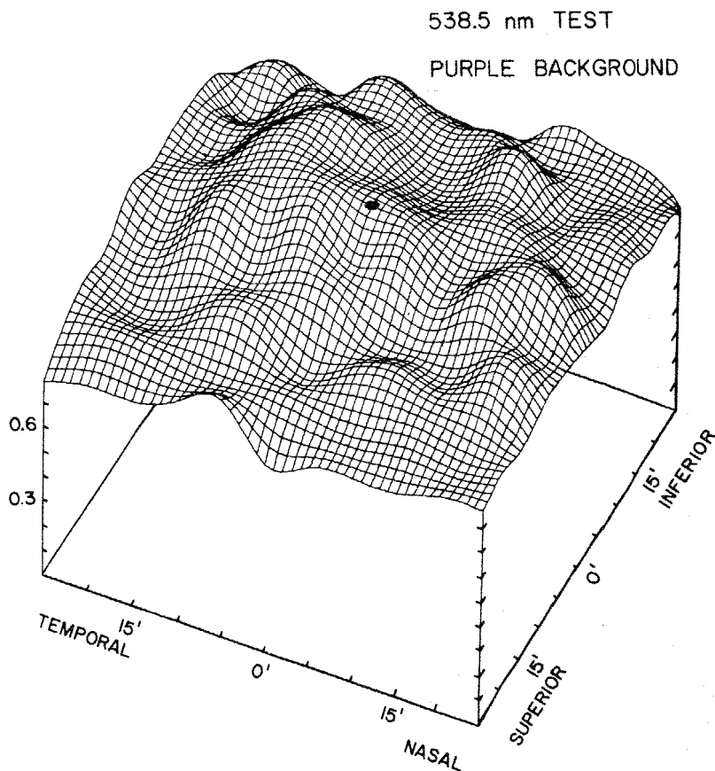
Fig. 5. Sensitivity map for D.R.W. using 538.5 nm 1.1' 50 msec test flash against a 3.4 log td, purple (Wratten 35) background. A value of 0.0 corresponds to 4.4 log quanta/flash.
