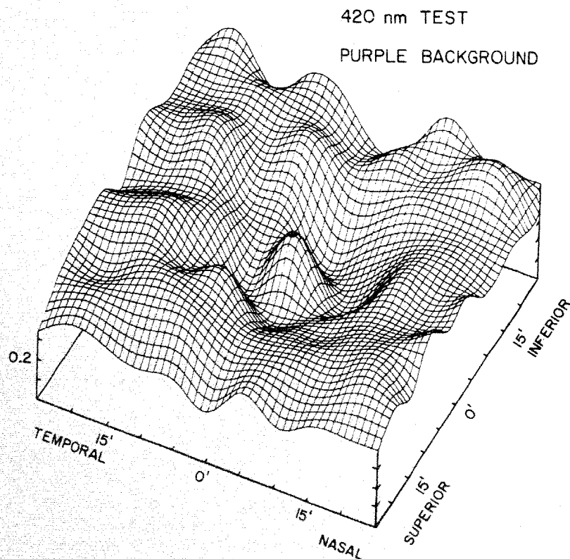
Fig. 4. Sensitivity map for D.R.W. using a 1.1', 420 nm, 50 msec test flash presented against a 3.4 log td, purple (Wratten 35) background. A value of 0.0 corresponds to 6.1 log quanta/flash.
