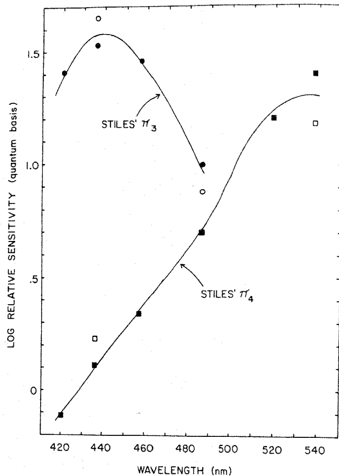
Fig. 2. Observer D.R.W.: Solid circles show the log relative sensitivity (quantum basis for a 50 msec test flash at an eccentricity of 35' presented against a 2.8 log td, 584 nm background. The data are fit with Stiles' \pi_3 . Solid squares show the log relative sensitivity for the test flash presented against a 3.4 log td, Wratten 35 background fit with Stiles' \pi_4 . Observer A.L.N.: Open circles show log relative sensitivity to two wavelengths for a 25 msec, 15' test flash at an eccentricity of 29 min presented against a 4.1 log td, 584 nm background.
