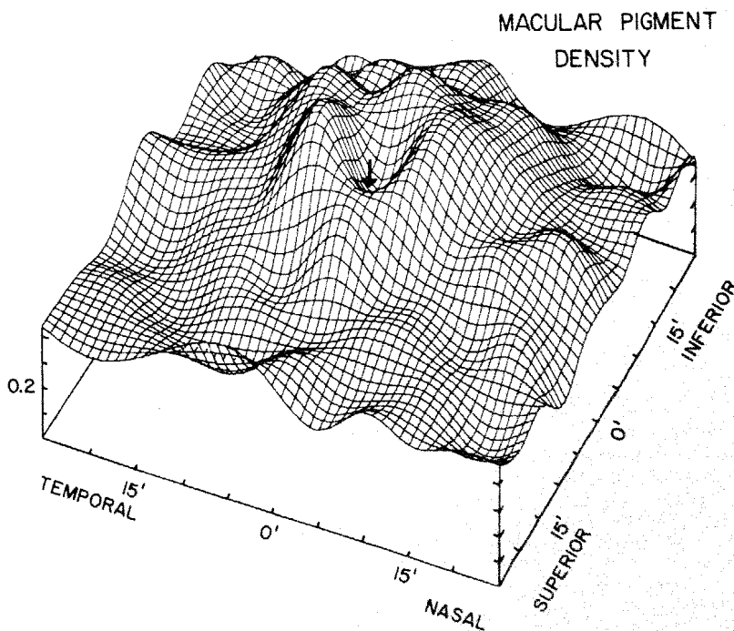
Fig. 6. Distribution of macular pigment density at 420 nm for D.R.W. calculated by subtracting log sensitivity values of Fig. 4 from those of Fig. 5 (G cone sensitivity with 420 nm test from G cone sensitivity with 538.5 nm test). Hatchmarks along side of figure represent density divisions of 0.1 log units.
