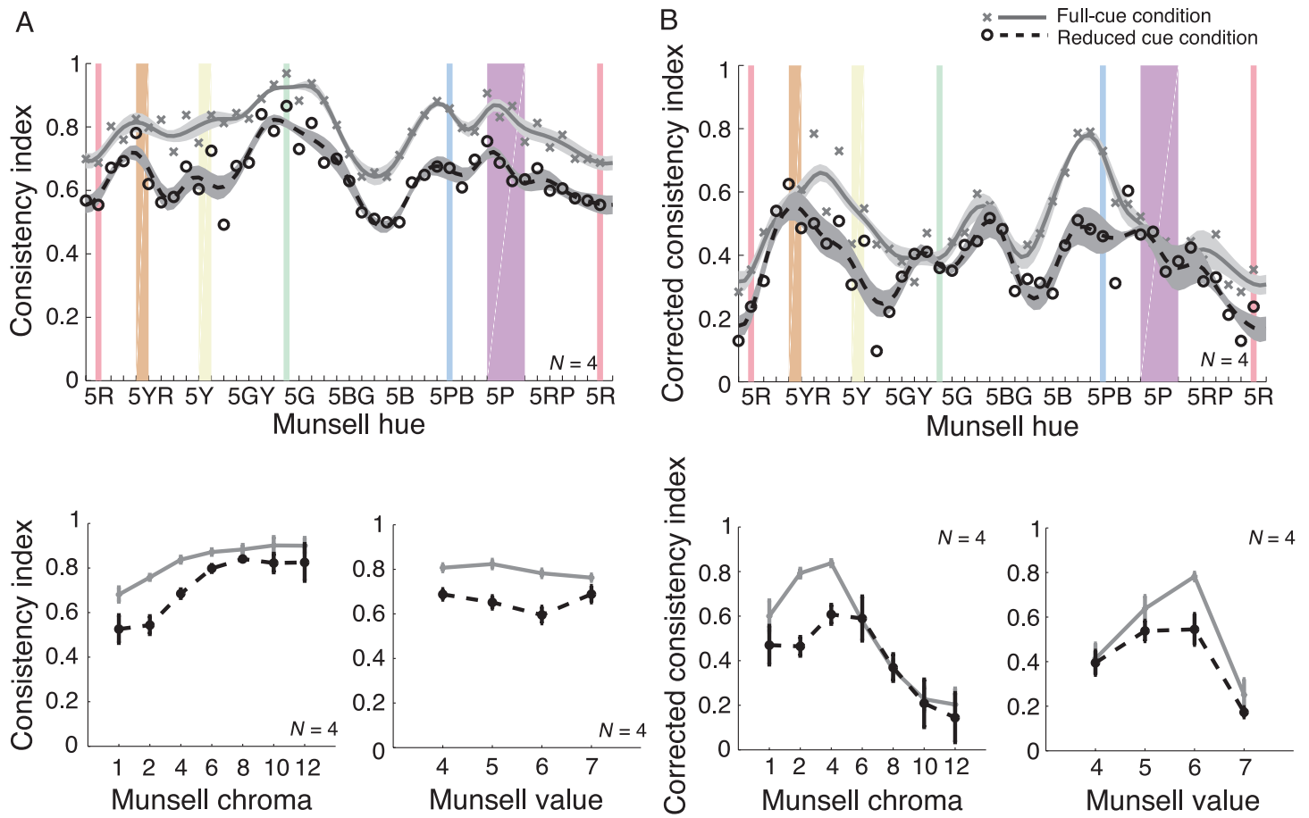
Figure 5. A: Uncorrected naming consistency indices for full-cue illuminants (gray curve) and reduced-cue illuminants (black dashed curve) are plotted as a function of Munsell hue (top panel), Munsell chroma (lower left) and Munsell value (lower right). Vertical bars in the upper panel indicate the range of prototypical hues. The smooth curves drawn through the data points were derived by averaging over two adjacent hues and interpolating between these averages. Shaded areas around the curves in the upper panel, and error bars in the lower panels indicate the standard errors of the means. B: The corrected naming consistency indices are plotted for Munsell hue (top), chroma (lower left) and value (lower right). Details as in A.
