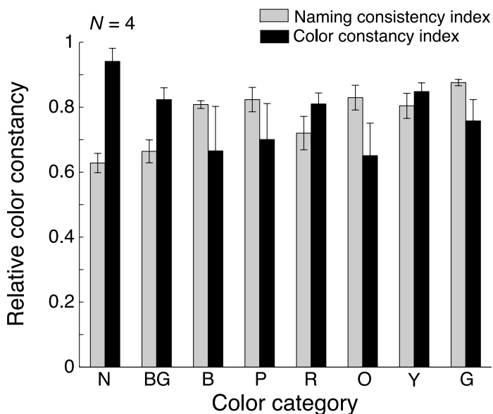
Figure 10. Comparison between the color constancy index and the uncorrected naming consistency index. Black bars plot color constancy calculated from the gray category centroids (Equation 1) and from the chromatic category boundaries (Equation 2). Gray bars plot naming consistency across illuminants. Color categories are indicated on the x-axis as follows: N: neutral; BG: turquoise; B: blue; P: purple; R: red; O: orange; Y: yellow; G: green.
