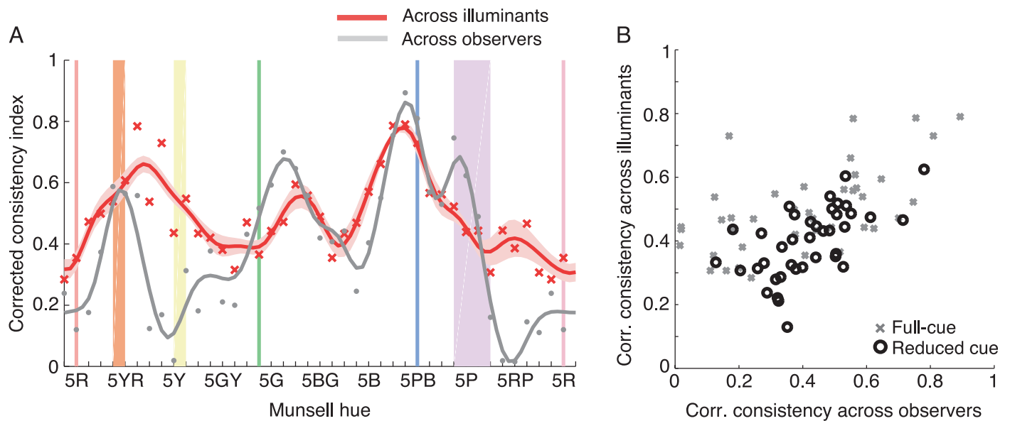
Figure 7. Comparison between naming consistency across illuminants and naming consistency across observers. A: Corrected naming consistency as a function of Munsell hue. Red crosses and the red curve plot naming consistency across illuminants. Gray circles and the gray curve plot naming consistency across observers for the neutral illuminant. Vertical bars indicate the range of prototypical hues. B: Corrected naming consistency across observers is plotted against consistency across illuminants for the full-cue (gray crosses) and reduced-cue (black circles) conditions. Each point indicates one Munsell hue, collapsed over saturation and lightness.
