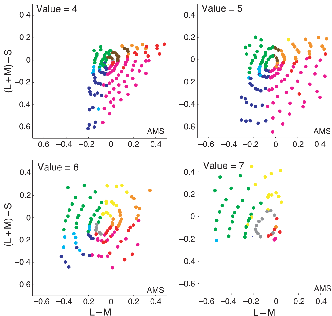
Figure 2. Naming data for subject AMS under the neutral full-field illuminant. Munsell chip chromaticities are plotted in the isoluminant plane of DKL color space. Chips with Munsell values 4 and 5 are plotted in the top row, and chips with values 6 and 7 in the bottom row. Symbol color denotes the color name given to a particular chip.
