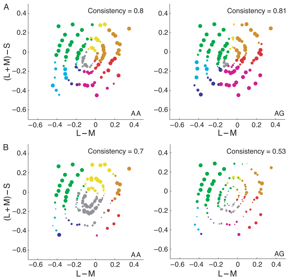
Figure 3. Naming consistency over illuminants for observer AA (left column) and AG (right column). The stimulus collection at value level 6 is plotted in the isoluminant plane of the DKL color space. Symbol size indicates the amount of consistency. A: Full-cue viewing condition. B: Reduced-cue viewing condition.
