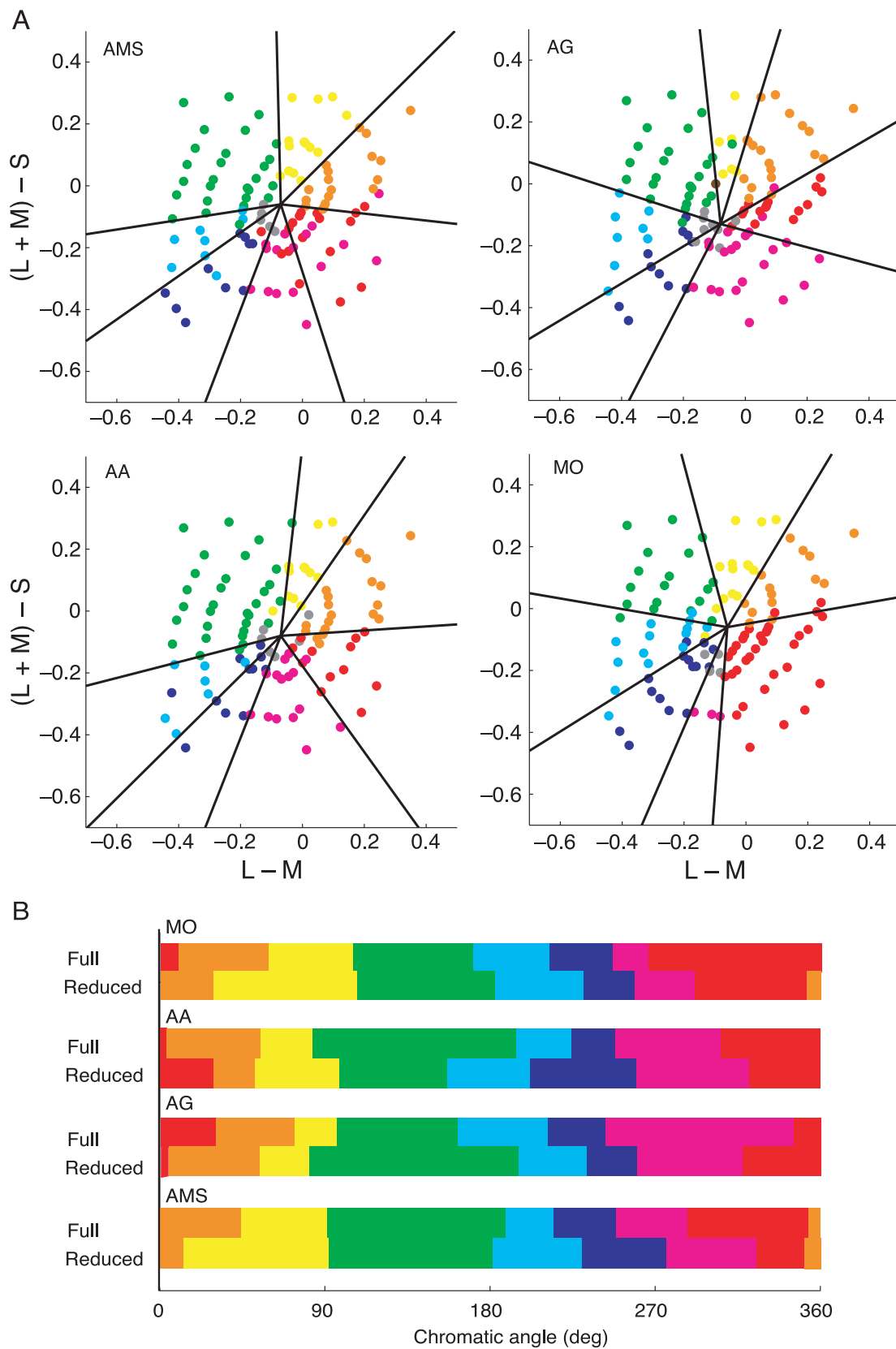
Figure 8. A: Chips with Munsell value 6 under the neutral illuminant are plotted in the isoluminant plane of DKL color space. Each quadrant is naming data for one subject in the baseline condition. Color categories are indicated with symbol colors. Black lines are best fitting category boundaries. B: Categories under neutral illumination are plotted as the color angles in the isoluminant plane between 0 and 360 degrees for all observers, and for the full-cue and reduced-cue viewing conditions.
