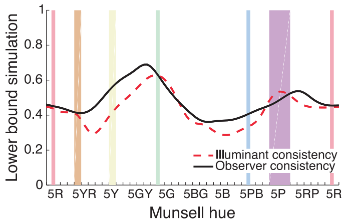
Figure 4. Lower bound simulation for consistency across illuminants (dashed red curve) and across observers (solid black curve) plotted for Munsell hue. The smooth curve was derived by averaging simulated values over two adjacent hues and interpolating between these averages. Vertical bars indicate the range of prototypical hues (from left to right red, orange, yellow, green, blue, purple, red).
