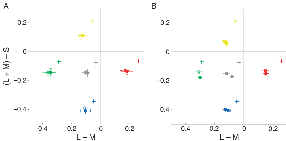
Figure 9. Achromatic points averaged over stimulus value in the full-cue (A) and reduced-cue (B) viewing conditions. Filled circles denote gray category centroids under the neutral and four chromatic illuminants; open squares denote the convergence points of the fitted boundaries under the five illuminants. Error bars are standard errors of the mean. Crosses denote the average chromaticity of the whole stimulus collection under each of the illuminants. Illuminant chromaticities are indicated by symbol colors.
