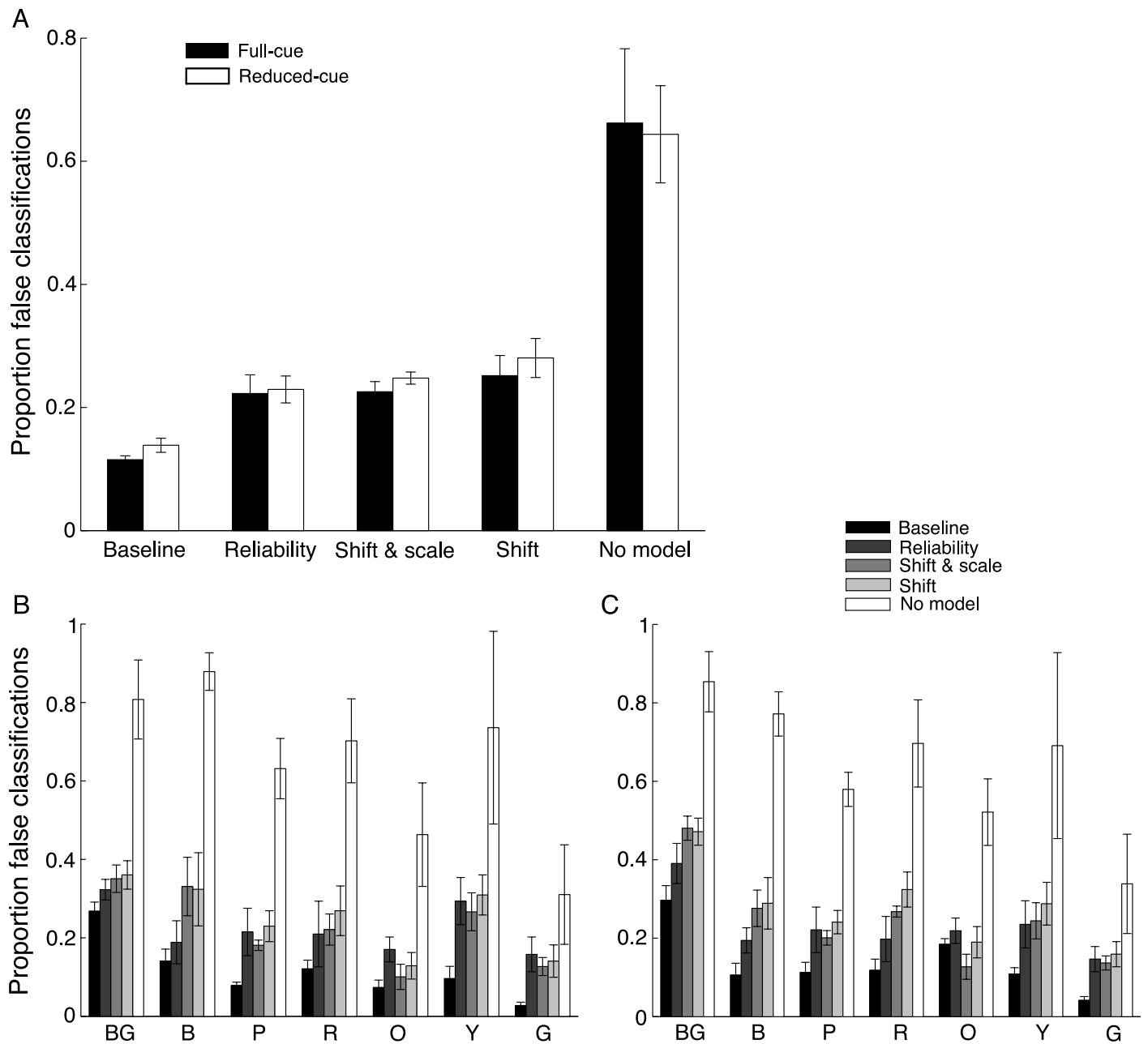
Figure 11. Boundary fit errors. A: Errors pooled over categories for the full-cue (black bars) and reduced-cue (white bars) viewing conditions for value level 6. B: Errors shown by category for the full-cue conditions. C: Errors shown by category for the reduced-cue conditions. Error bars show the standard errors of the means over illuminants ( N = 5 ). Baseline: average errors of the boundary fits in each illuminant condition separately. Reliability: average errors from fitting boundaries over the two repetitions in each illuminant condition. Shift & scale: fitting baseline boundaries to the test conditions with two shift and two scale parameters. Shift: fitting baseline boundaries to the test conditions with two shift parameters. No model: superimposing baseline boundaries on the test data without transformations. Color categories are indicated on the x-axis as follows: BG: turquoise; B: blue; P: purple; R: red; O: orange; Y: yellow; G: green.
