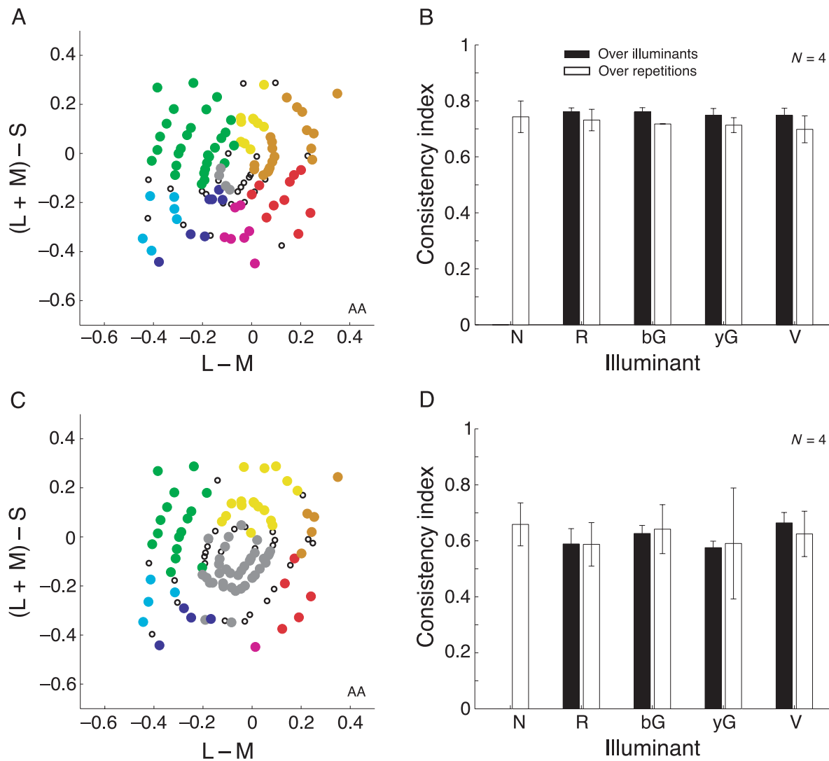
Figure 6. A: Naming consistency under the neutral illuminant over two repetitions for observer AA in the full-cue condition. Chips that were classified in the same category over repetitions are indicated with filled symbols. B: Uncorrected naming consistency across repetitions and across illuminants for the five full-field illuminants. Error bars show the standard errors of the mean. Illuminants are indicated on the abscissa as follows: N: neutral; R: red; bG: bluish-green; yG: yellowish-green, V: violet. C: Naming consistency under the neutral illuminant over two repetitions for observer AA in the reduced-cue condition. D: Uncorrected naming consistency for the reduced-cue illuminants.
