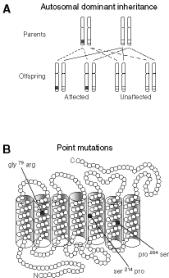
Figure 1.18: Tritan defects. (A) Autosomal dominant inheritance. On average, one-half of the offspring of a heterozygotic parent will inherit the disorder. An open square on the q-arm of chromosome 7 indicates a normal S-cone pigment gene; a filled square, one carrying a missense mutation. (B) Schematic representation of the S-cone pigment showing the locations of three identified amino-acid substitutions.
