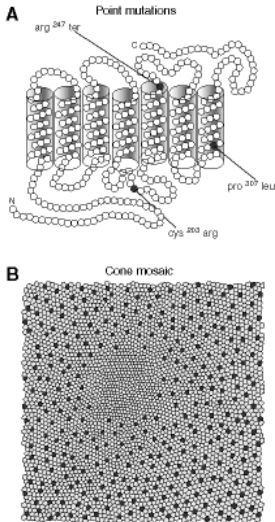
Figure 1.17: Blue-cone monochromacy. (A) Schematic representation of a 5M-3L hybrid pigment showing the locations of identified point mutations. The seven \alpha -helices are shown embedded within the membrane. N and C denote amino- and carboxyl-termini, respectively. (B) The cone mosaic of the rod-free inner fovea of an adult human retina at the level of the inner segment; computer altered to simulate the consequences of blue-cone monochromacy. The positions of the S-cones are shown in black; the positions of the M- and L-cones, in white to indicate the lack of a functioning cone pigment. See legend to Fig. 1.1C for other details.
