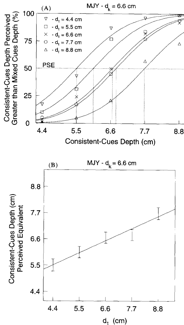
FIGURE 7. (A) Psychometric functions from a depth comparison experiment involving texture and motion cues (Young et al. , 1993). Each curve represents a different value of d_t , and d_k is fixed throughout. The abscissa shows the value of d for the comparison, consistent-cues stimulus, and the ordinate shows the probability that the consistent-cues stimulus was perceived as having greater depth. As the discrepant value of d_t is increased, the curves slide rightward. (B) The points of subjective equality estimated from (A) along with confidence limits. The data are consistent with a linear trend. The slope of the curve provides an estimate of \alpha_t = 0.46 .
