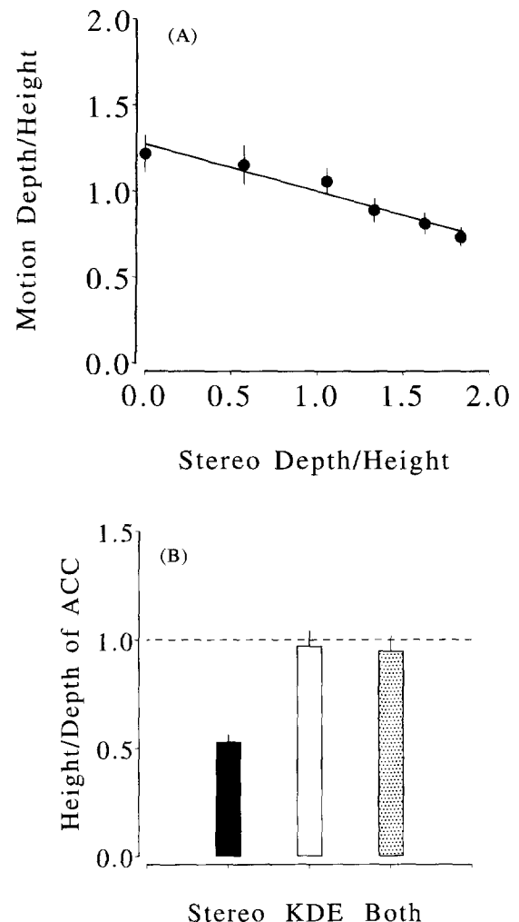
FIGURE 8. (A) Apparently circular cylinder data for surfaces with incongruent depths specified by kinetic depth and stereo (from Johnston et al. , 1994). The data points show the depth/height portrayed by stereo and by motion which resulted in a cylinder which appeared circular to the subjects. Viewing distance was 200 cm. (B) Portrayed height/depth for cylinders which appeared circular (data shown are an average over three subjects). For stereo alone, depth is underestimated at this viewing distance (i.e. an exaggerated amount of depth is required for the cylinder to appear circular, hence height/depth is < 1 ). For KDE alone and for the combination, perception is veridical.
