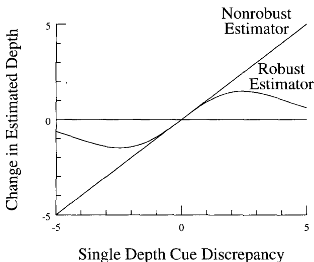
FIGURE 4. A representative influence curve for a robust statistical estimator. As a single cue specifies an increasingly discrepant amount of depth relative to other cues, at first overall perceived depth changes accordingly, but eventually the discrepant cue is downweighted. A nonrobust estimation procedure such as a simple average would predict the linear function.
