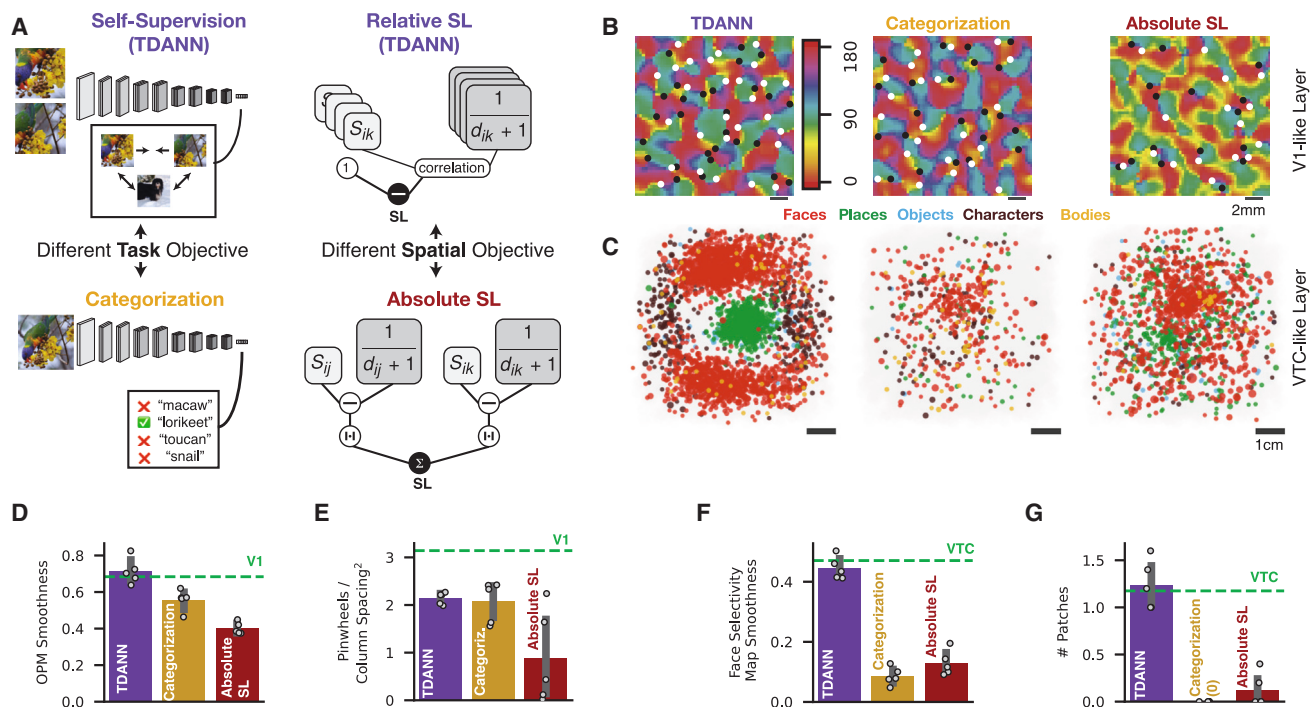
Figure 5. Self-supervision and scalable spatial constraints underlie the emergence of functional organization
